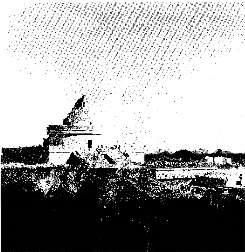
(b) The Caracol, an observatory at Chichen Itza, Yucatan
