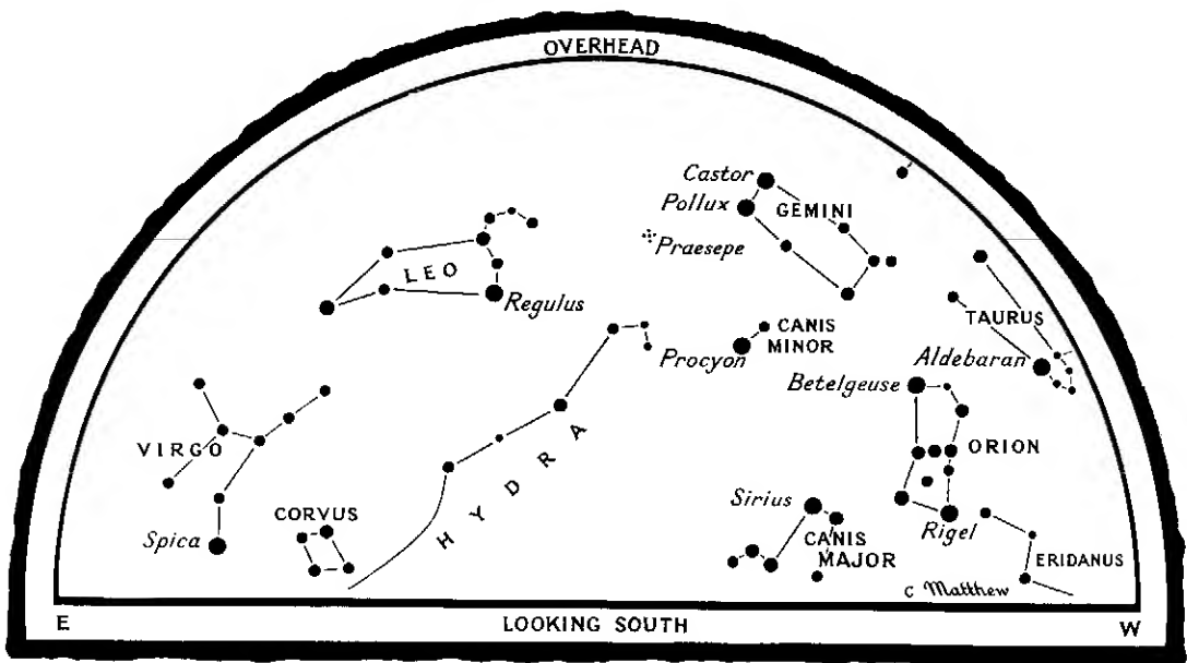
1. Night sky at latitude of London at mid-March
