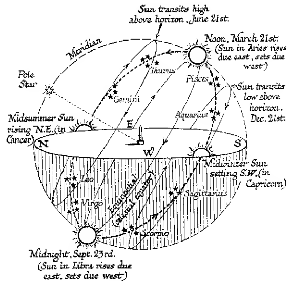
5 (a) Apparent diurnal motion of the stars (b) The changing heavens
