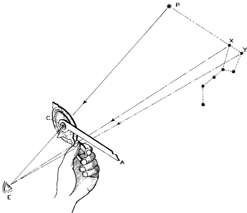
(b) The stars marked X and Y are the clock stars of the Great Bear. P is the Pole Star
