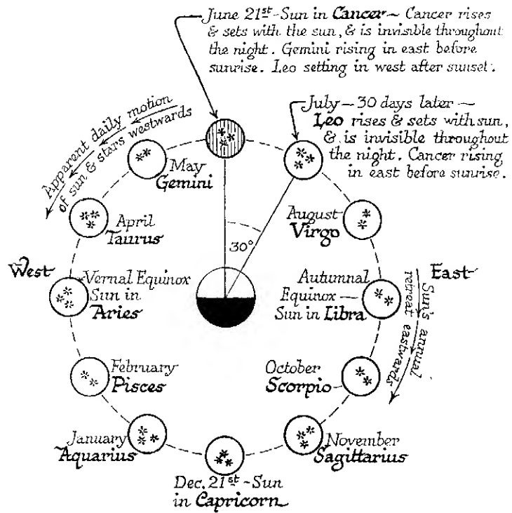
7. The sun's (apparent) annual retreat through the zodiacal constellations (The South Pole of the earth is nearest to you in the figure.)
